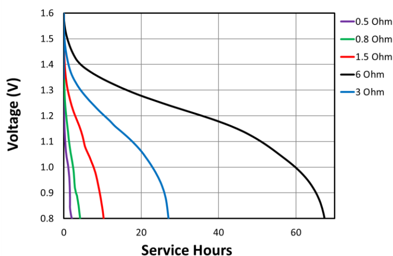
Constant Resistance
