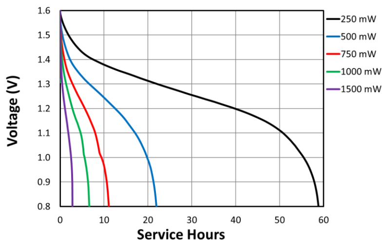
Constant Power
