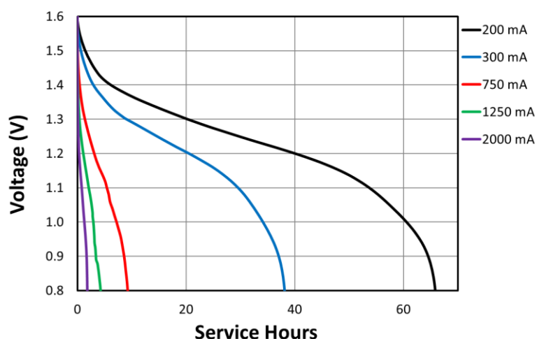
Constant Current
